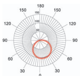
QUADRANT WALL
